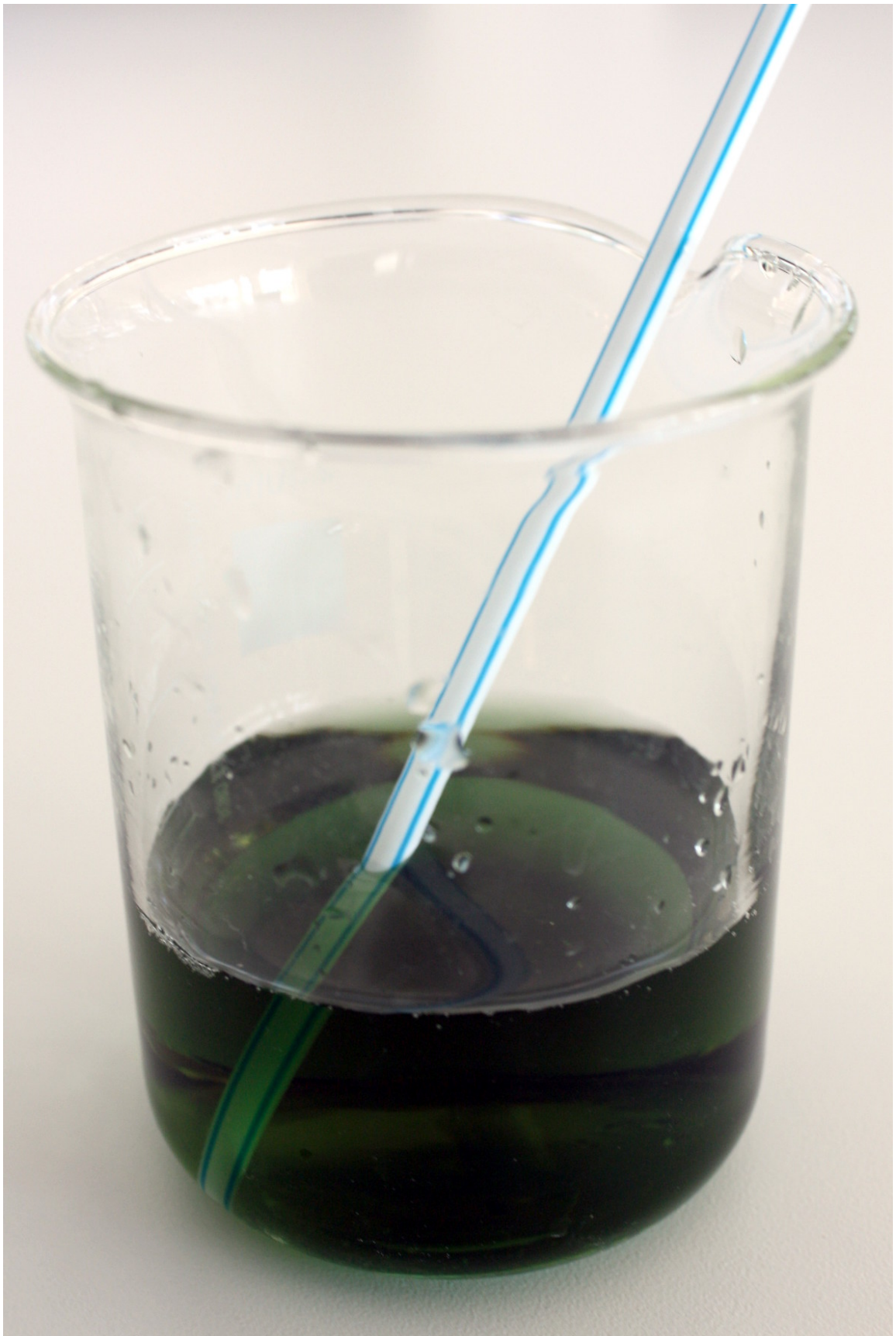
Figure 11: The water after the addition of some pH indicator has a pH value of 8.
