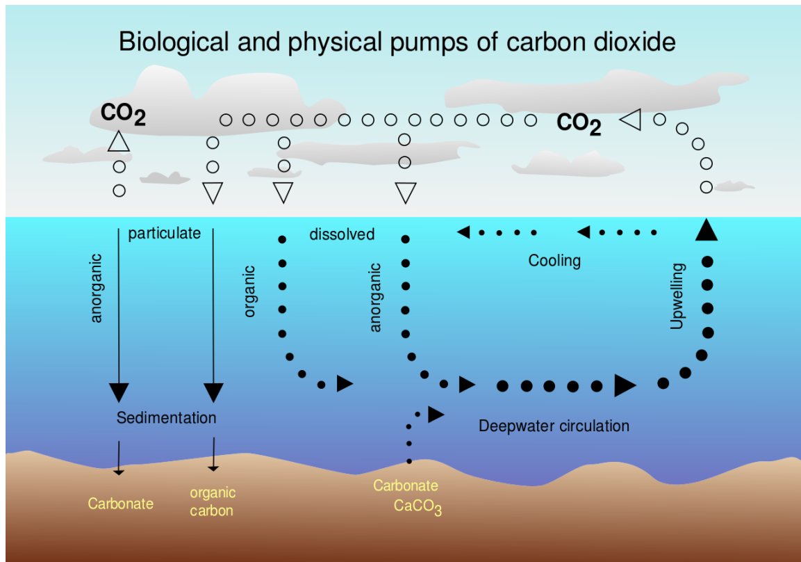
Figure 4: Air-sea exchange of carbon dioxide (McSush (modified), Hannes Grobe (original), https://commons.wikimedia.org/wiki/File:CO2_pump_hg.svg , https://creativecommons.org/licenses/by-sa/2.5/legalcode ).
