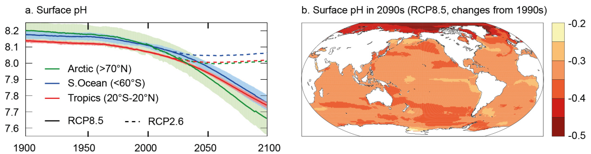
Figure 7: Past and projected evolution of oceanic surface pH levels. The models were calculated for the most optimistic (RCP2.6, Representative Concentration Pathways) and the most pessimistic scenarios (RCP8.5) for the evolution of atmospheric CO 2 . (a) Time-series of surface pH shown as the mean (solid line) and range of models (filled), given as area-weighted averages over the Arctic Ocean (green), the tropical oceans (red) and the Southern Ocean (blue). (b) Map of the median model's change in surface pH from 1990 to 2090 (IPCC Report, 2013, Working Group I, Chp. 6, p. 532, permission for reproduction granted).
