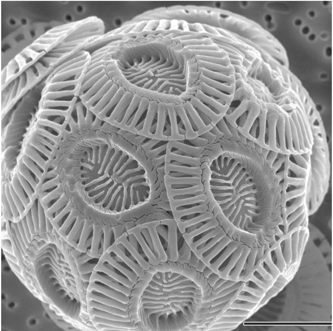
Figure 9: Image of a single coccolithophore cell produced with a high-resolution scanning electron microscope (Credit: Alison R. Taylor (University of North Carolina Wilmington Microscopy Facility) ( https://commons.wikimedia.org/wiki/File:Emiliana_huxleyi_coccolithophore_(PLoS).png ), https://creativecommons.org/licenses/by/2.5/legalcode ).
