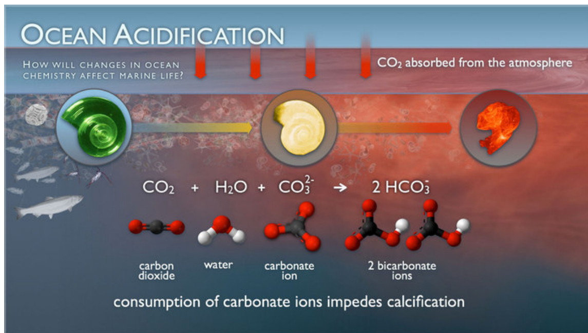
Figure 5: Illustration of how CO 2 dissolved in water consumes carbonate ions. It impedes calcification or may even lead to decalcification of sea shells (NOAA PMEL Carbon program, NAOO public domain).
