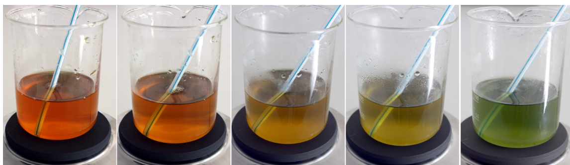
Figure 14: On heating the acidic liquid, the colour starts to change again. The acidification is reversed because carbon dioxide is driven out of the liquid. Warm water cannot store as much carbon dioxide as water at lower temperatures.
