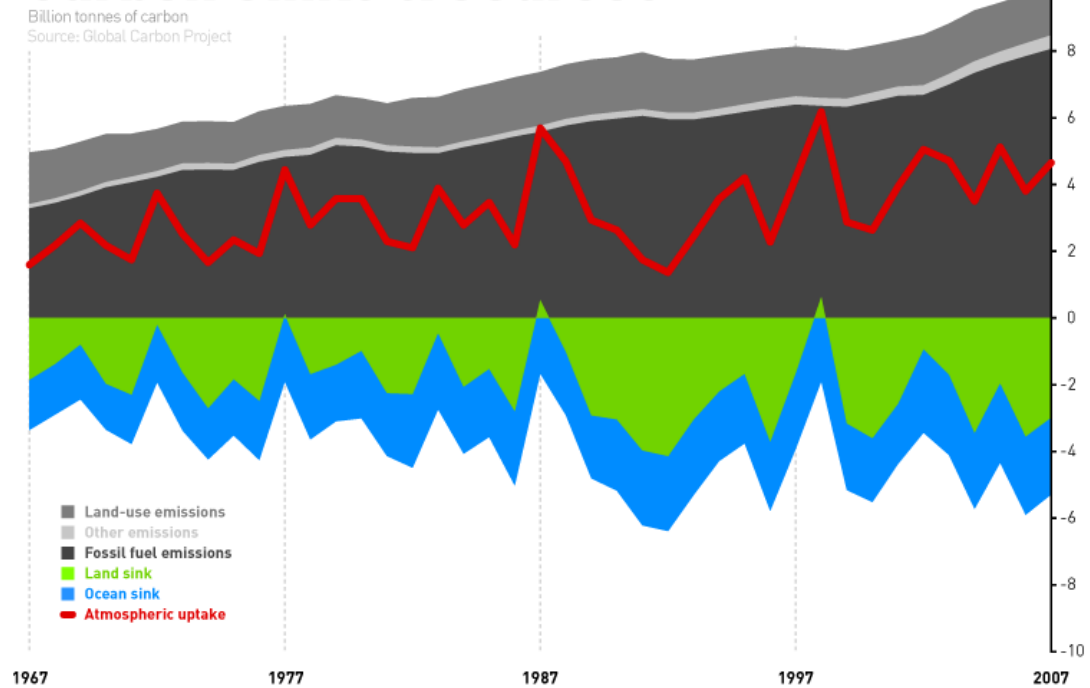
Figure 2: Evolution of the budget of carbon sinks and sources (climatesafety, https://www.flickr.com/photos/climatesafety/4745854611 , https://creativecommons.org/licenses/by-nc/2.0/legalcode ).
