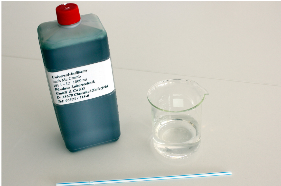
Figure 10: Items required for the first part of the activity.
