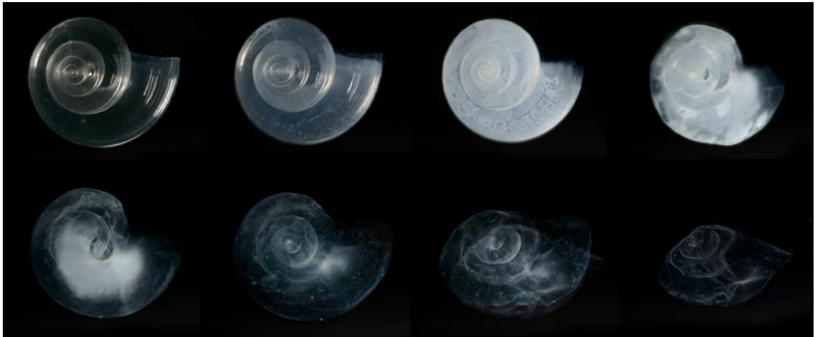
Figure 8: In laboratory experiments, the shell of this sea snail dissolved over the course of 45 days in seawater adjusted to an ocean chemistry projected for the year 2100 (Credit: NOAA Environmental Visualization Laboratory (EVL), https://commons.wikimedia.org/wiki/File:Pterapod_shell_dissolved_in_seawater_adjusted_to_an_ocean_chemistry_projected_for_the_public_domain ).
