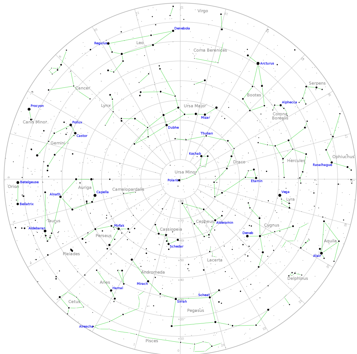
Figure 15a: Star chart of the Northern Hemisphere
