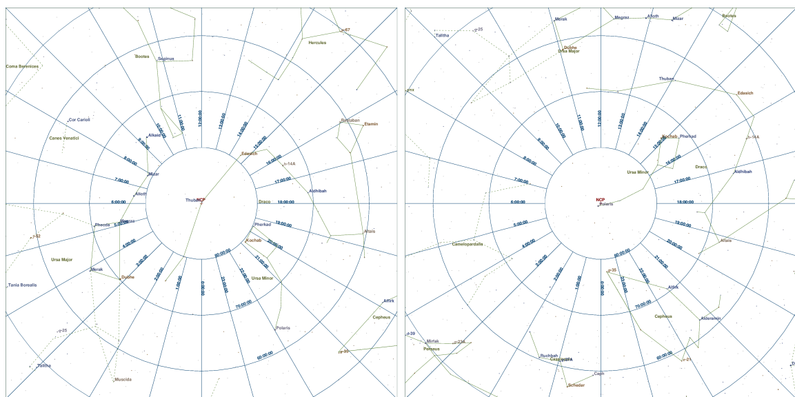
Figure 7: Star charts of the northern celestial pole region for the years 2750 BCE and 2016 CE (Credits: own work, created with XEphem Version 3.7.6, produced by Elwood C. Downey and distributed by the Clear Sky Institute Inc., Solon, Iowa, USA, http://www.xephem.com ).
