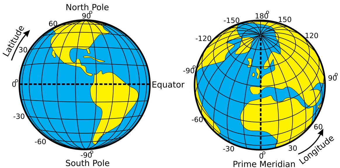
Figure 2: Illustration of how the latitudes and longitudes of the Earth are defined (Credits: Peter Mercator, djexplo, CC0).
