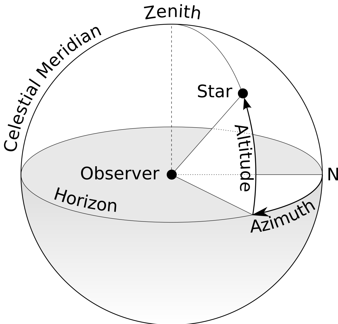
Figure 5: Illustration of the horizontal coordinate system. The observer is the origin of the coordinates assigned as azimuth and altitude or elevation (Credit: TWC Carlson, https://commons.wikimedia.org/wiki/File:Azimuth-Altitude_schematic.svg , 'Azimuth-Altitude schematic', https://creativecommons.org/licenses/by-sa/3.0/legalcode ).
