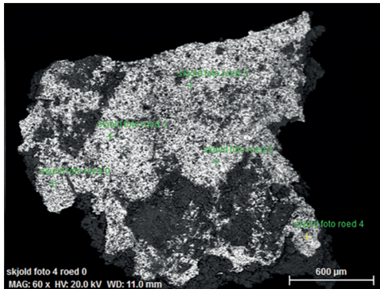
Fig. 24. Backscatter (BSE) picture of Baunegård-a. The BSE picture contains elemental information, as different elements are displayed as varying grayscales. The heavier the element the more signal it emits, i. e. highlighted areas on the picture. The picture therefore shows the distribution of the pigment as highlighted areas. The points marked on the picture were analysed with EDX.
