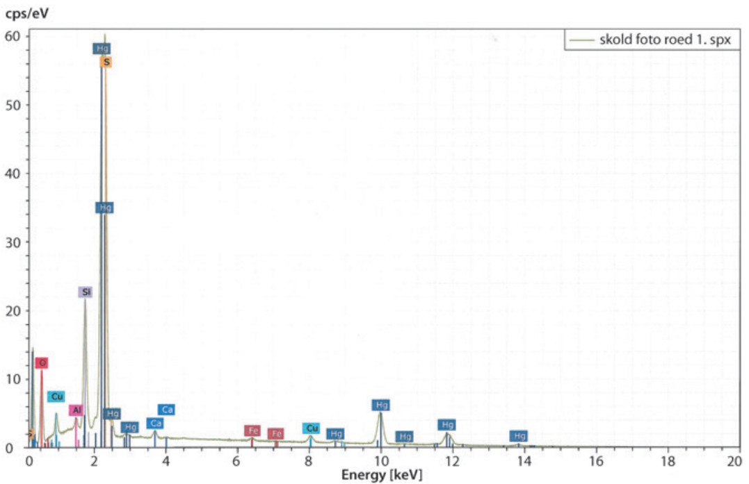
Fig 25. The spectrum from Baunegård-a, point skjold foto roed 1 (EDX analysis). The analysis shows the presence of cinnoba containing some trace elements deriving from the mineral or/and the surrounding soil.
