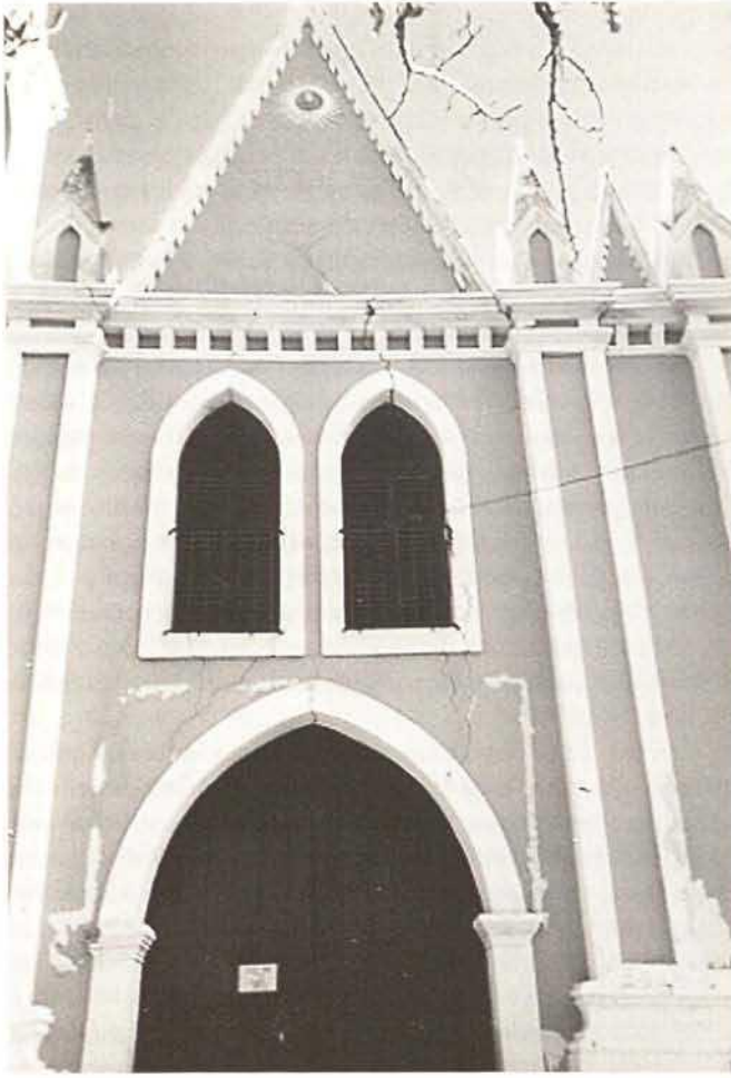
Coro, Iglesia de San Francisco, cracks and general damage due to movements of the earth
