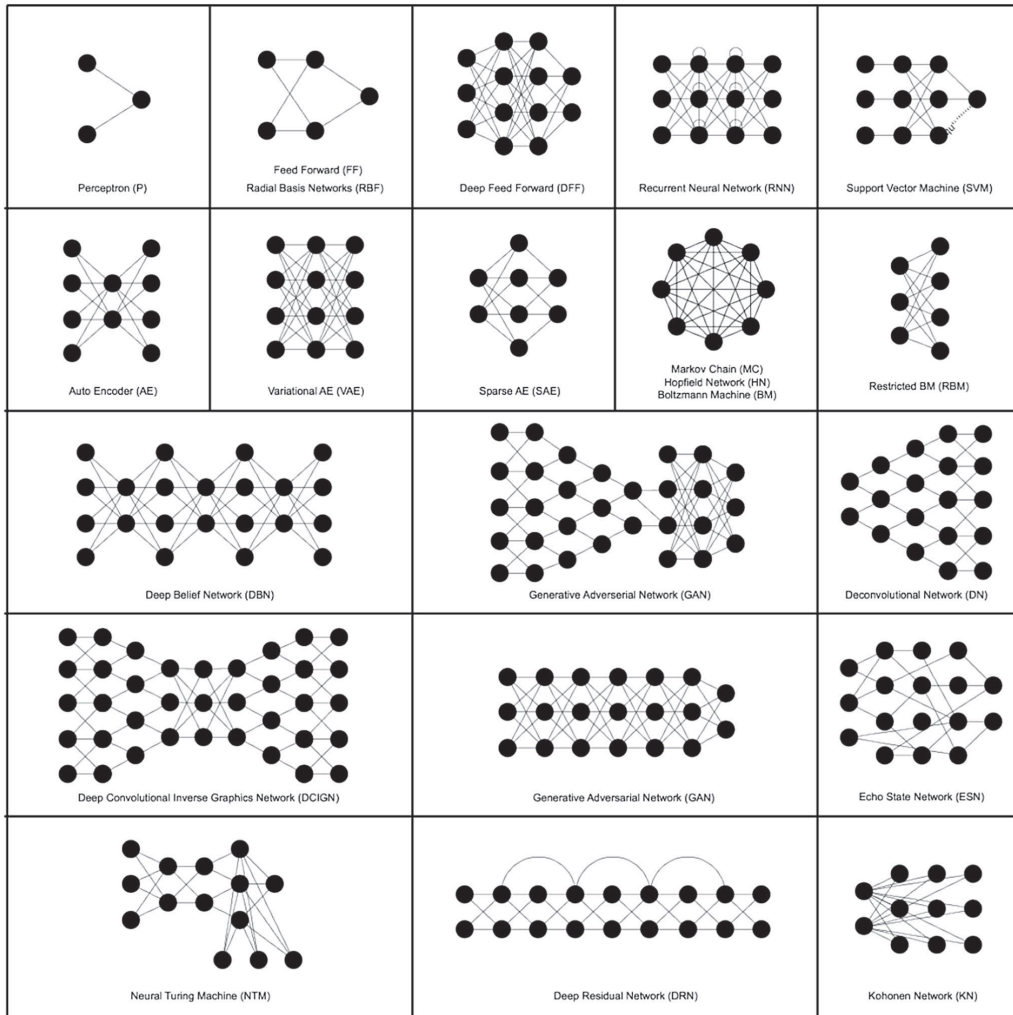
Fig. 4: Source: https://www.asimovinstitute.org/neural-network-zoo .
