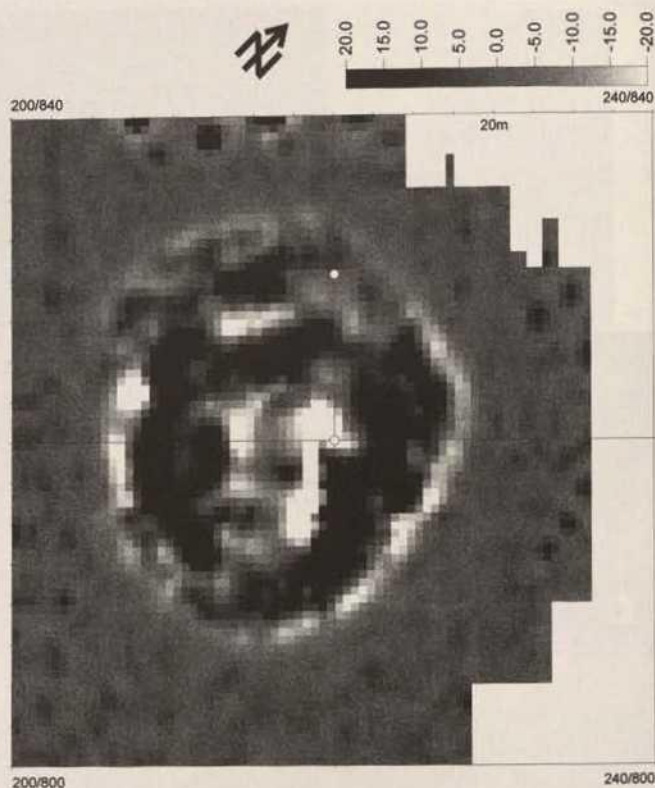
Fig. 4b. Ambrona-Dolmen de la Sima 1998. Resistivity diagram of the round barrow. Geoscan RM15-Advanced resistance meter with twin electrode, raster 0.5/0.5 m, dynamics -20.0/+20.0 units (original data 40.0/240.0 Ohm m), 20 m grid
