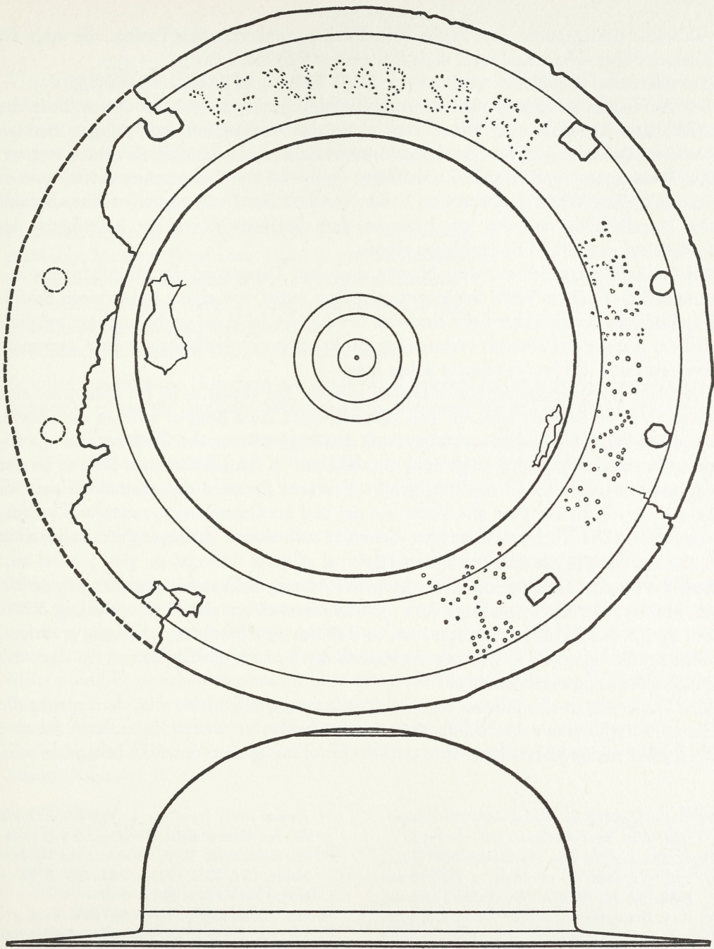
Abb. 4 Bronzeschildbuckel C. Fo. Mainz. Mus. Wiesbaden. M = 3:4.
