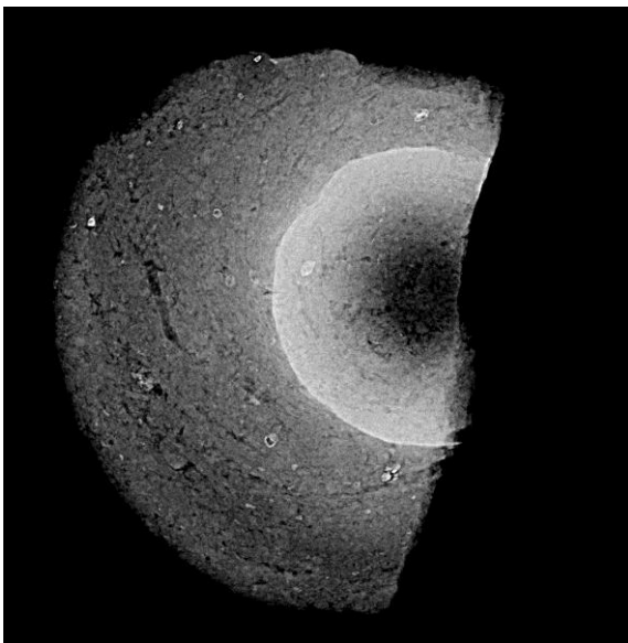
Figure 2c: Enhanced radiograph of a Middle Minoan IIB conical cup showing a diagonal alignment of voids characteristic of the wheel-throwing technique (Berg 2009: catalogue no 51).
