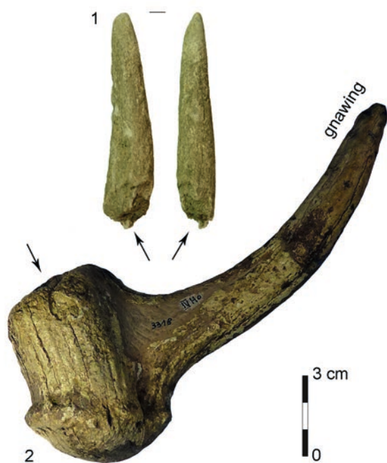
Fig. 7. Kammern-Grubgraben, AL3. Manufacturing debris from red deer antler. Removed tine (1) and removed basal section (2). Note chopped, circular notches (arrows). Repository Austrian Academy of Sciences. Photos S.J. Pfeifer.
