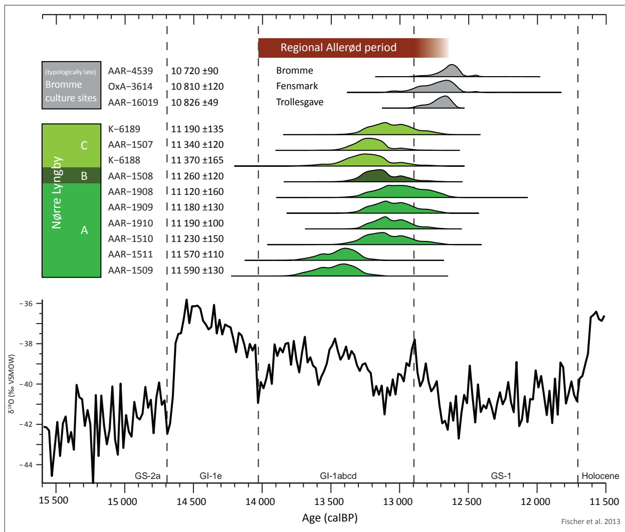
Fig. 19. Comparison of three AMS ^{14}C dates for activity sites from typologically late Bromme culture, dates for reindeer bones from Nørre Lyngby and climatic data from Greenland ice cores. The designations for the generally colder periods begin with GS (Greenland Stadial), while the names of the generally warmer periods begin with GI (Greenland Interstadial) (Björck et al. 1998; Blockley et al. 2012).
